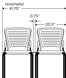
Armless - Ganging Dimensions
